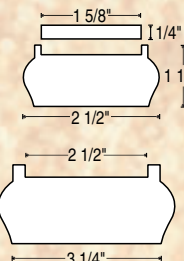
Colonial Sboerail
