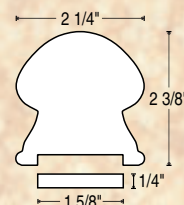
Southampton Handrail
