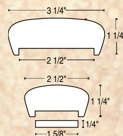
Colonial Handrail
